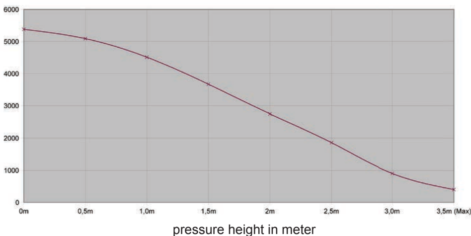
Liter/h Power curve 50W full load
